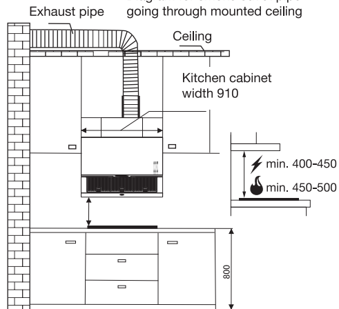
Diagram for smoke outlet pipe going through mounted ceiling
