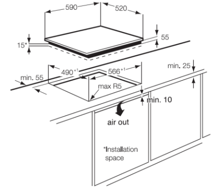
Induction hob over an oven
