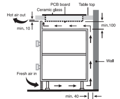
Induction hob over a drawer
