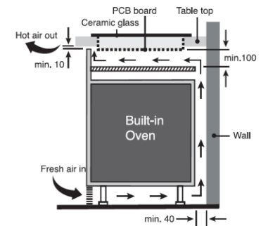
Induction hob over an oven
