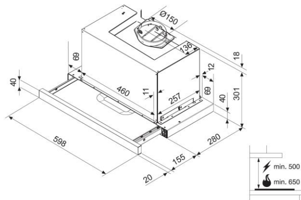
EFP60473OS
