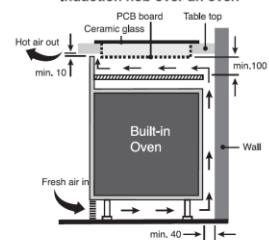
Induction hob over an oven
