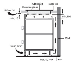
Induction hob over a drawer
